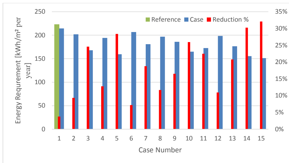
Figure 5. Energy requirement for different renovation packages. Case numbers on x-axis correspond to Table 5.
